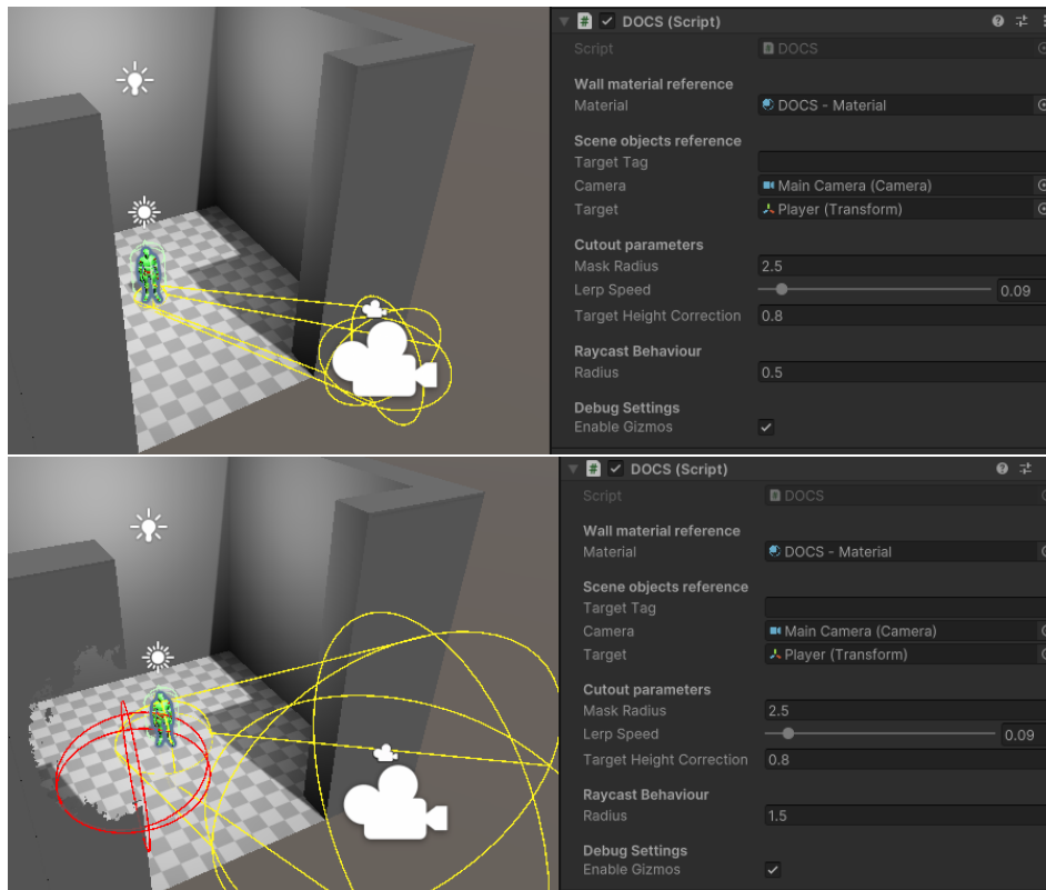
Fig. 4 – Radius of SphereCast set to 0.5f and 1.5f (exaggerated)
