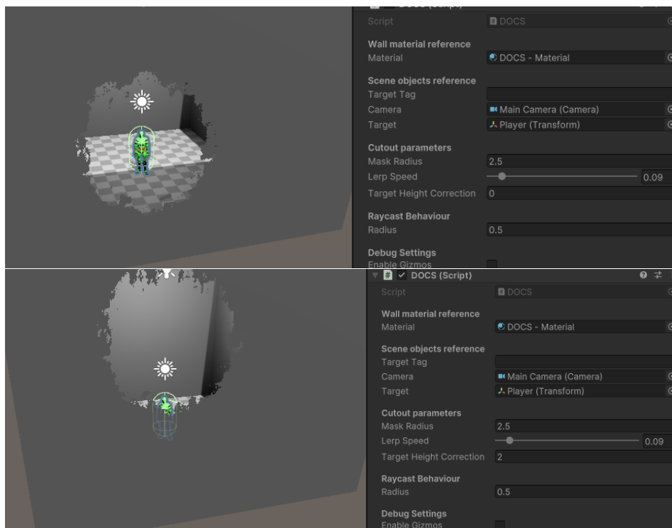
Fig. 3 - Target Height Correction set at 0.0f and 2.0f (exaggerated)
